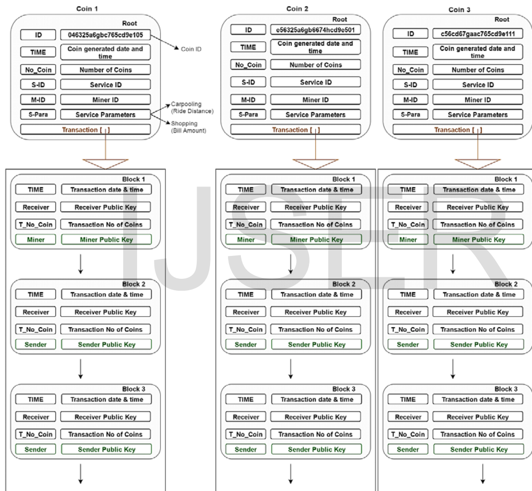
Figure B. 1 Coin Wise Blockchain Design
