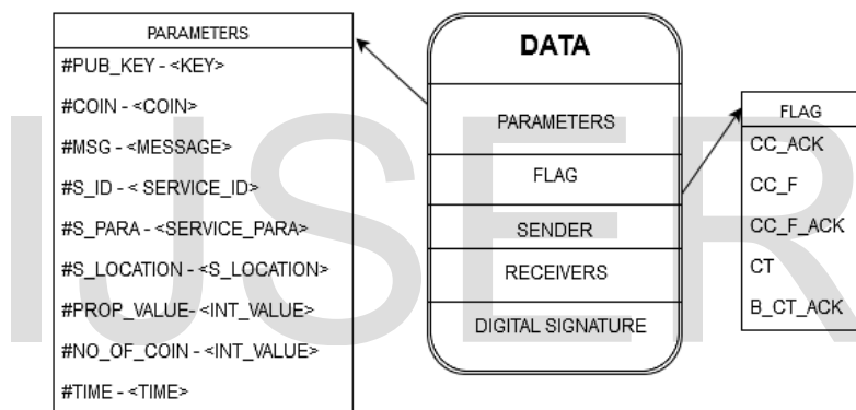
Figure 3.3.3 Protocol Design: 'DATA' Protocol
