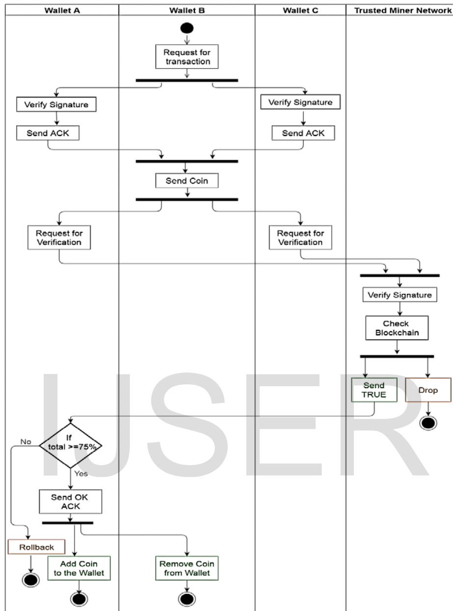
Figure 5.2.1 Double Spending Evaluation
