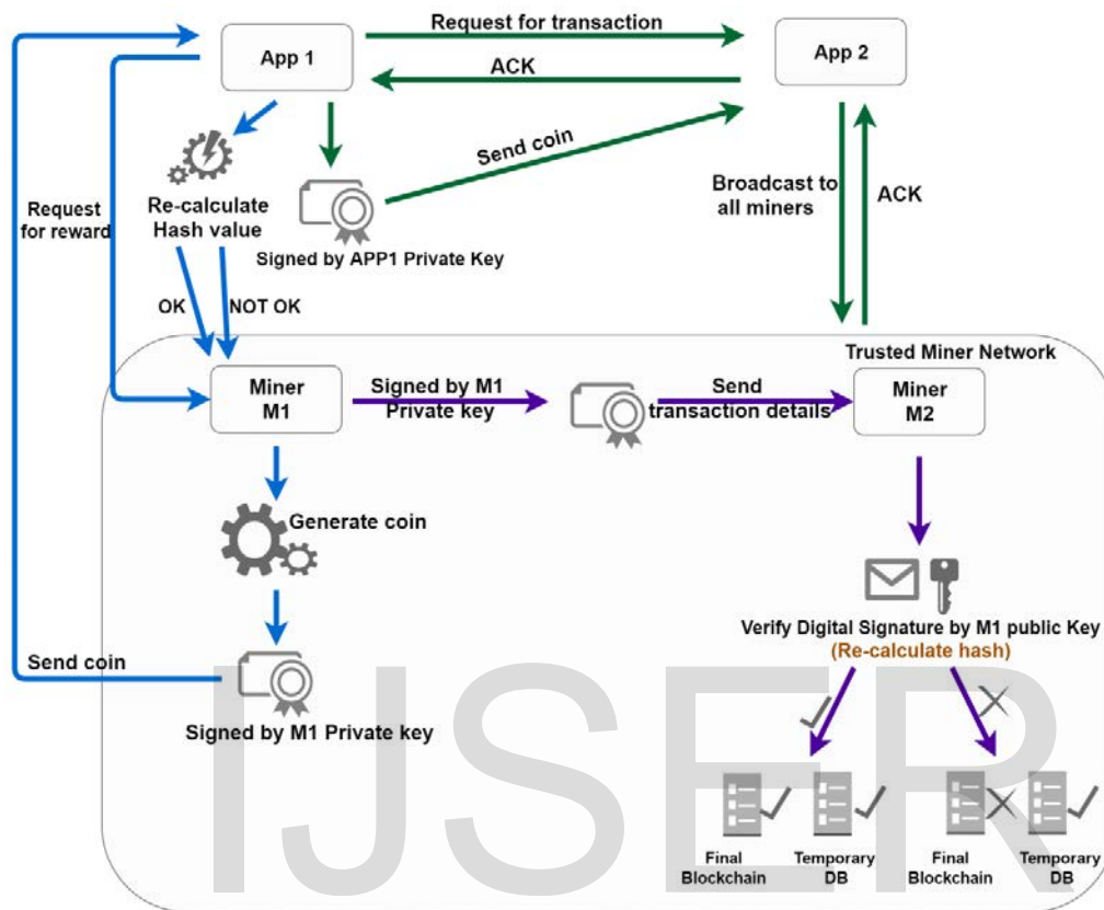
Figure 3.4.1 Transactions Overview in a Common Payment Platform
