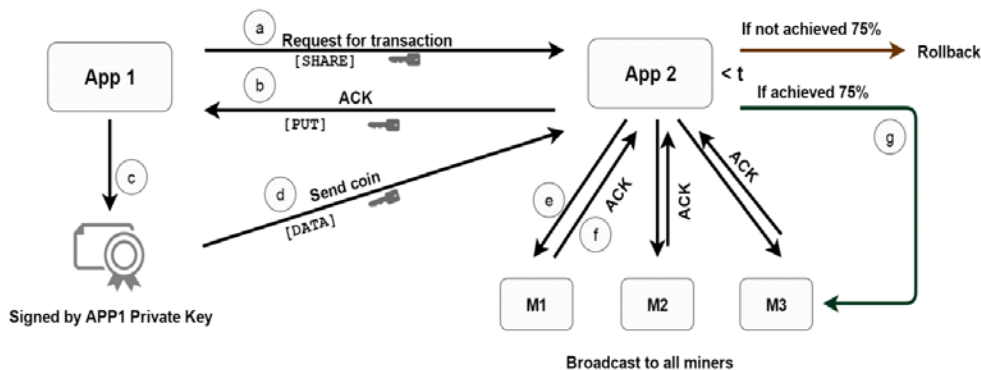
Figure 3.4.4 Scenario C:App-App Transaction Verification Model
