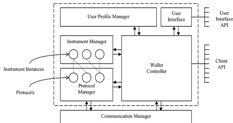
Figure 2.2.2 The SWAP Generalized Digital Wallet Architecture
