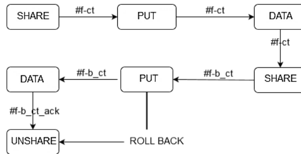
Figure 4.2.2 App to App Protocol Implementation
