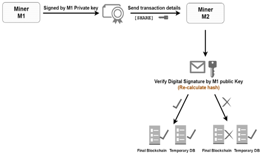
Figure 3.4.3 Scenario B: Miner-Miner Transaction Verification Model
