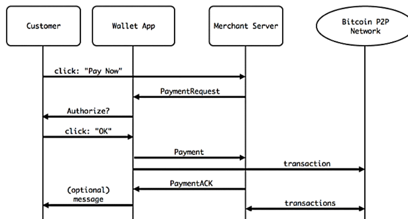
Figure 2.4.1 Overview of the BIP Payment Protocol
