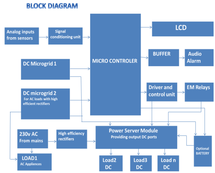
Fig 1: Block Diagram of DC Micro-grid
