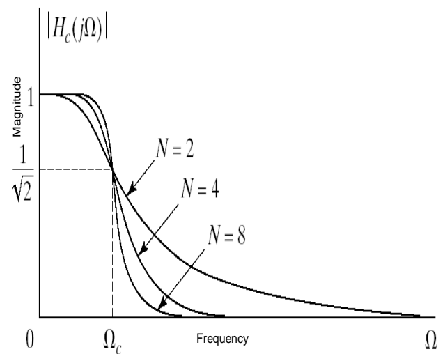
Fig. 3(d) Frequency response of Butterworth filter
