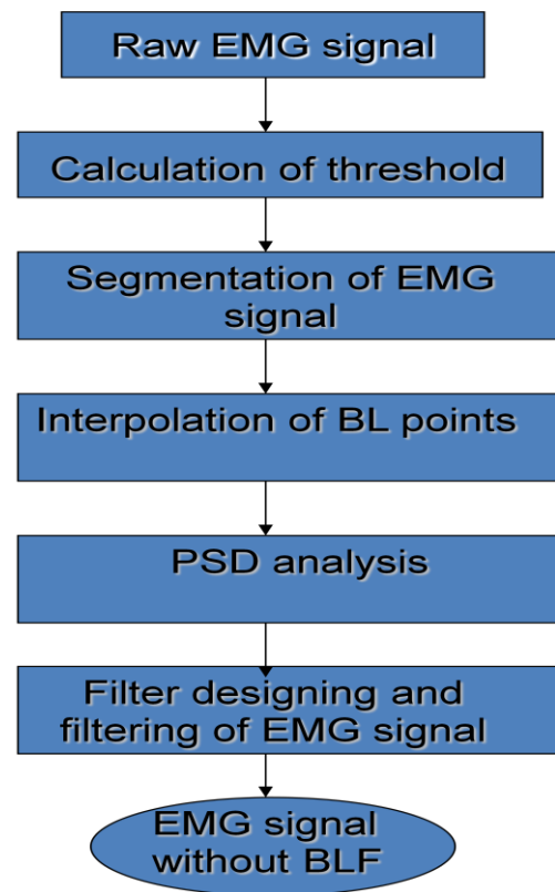
Figure3. Flow chart of filter designing method
