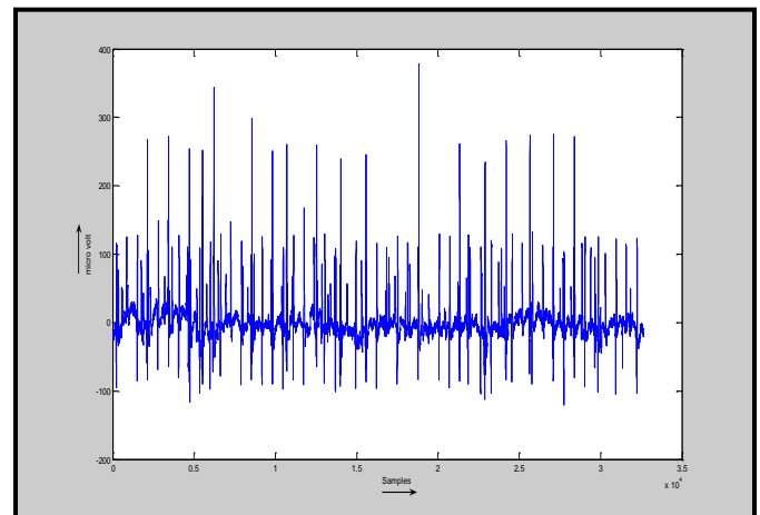
Figure 2(a). EMG signal with BLF
