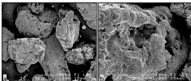
Fig. 7. SEM photomicrographs of completely reduced iron powder at 180 min and at 1050°C.
