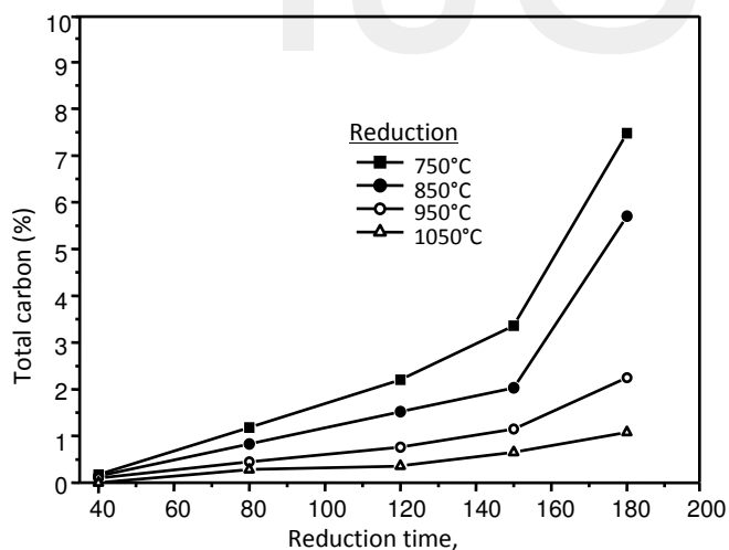
Fig. 3. Evolution of total carbon content in reduced iron powders with temperature and reduction time.
