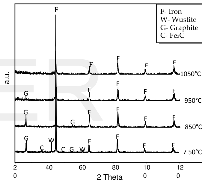
Fig. 4. X-Ray spectra of the reduced iron powders at various temperatures and 180 min.
