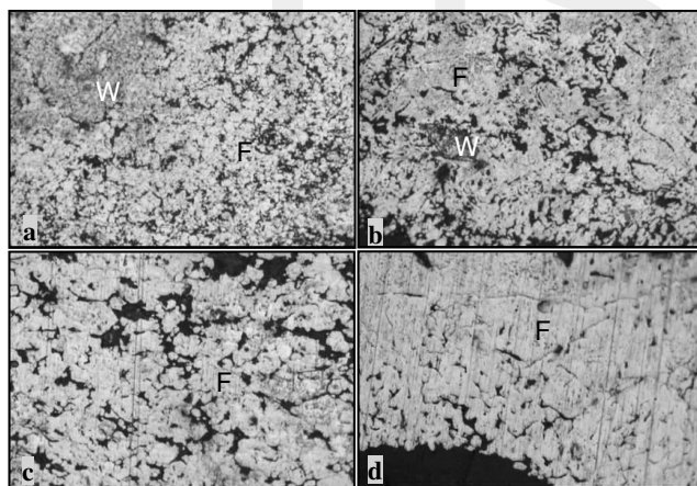
Fig. 6. Photomicrographs of reduced iron powders (x220) at 180 min and at (a) 750°C, (b) 850°C, (c) 950°C and (d) 1050°C. W: wustite F: iron
