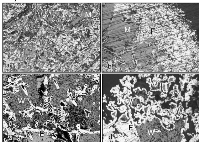
Fig. 5. Photomicrographs of reduced iron powders (x220) at 40 min and at (a) 750°C, (b) 850°C, (c) 950°C and (d) 1050°C. M: magnetite, W: wustite, F: iron
