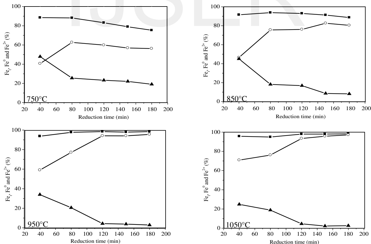
Fig. 2. Evolution of \blacksquare Fe total , \circ Fe 0 and \blacktriangle Fe 2+ content in reduced iron powders with temperature and reduction time.
