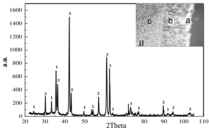
Fig.1. Oxide scale formed on the mill scale: (I) XRD spectra (II) cross-section microstructure. (1) Hématite (2) Magnétite (3) Wustite
