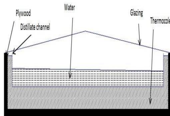
Fig. 1 –Single basin double slope solar still
