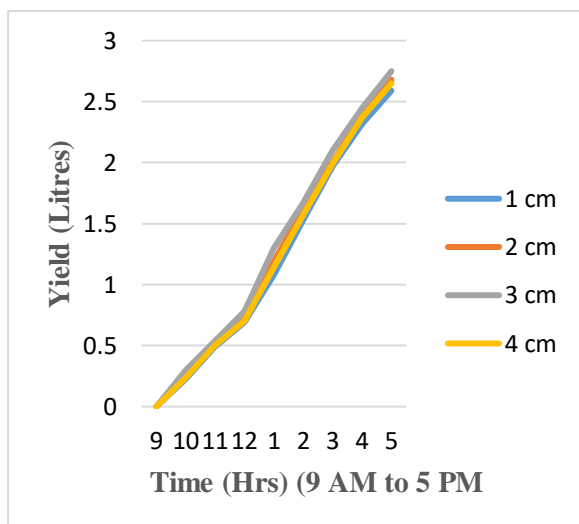
Fig. 6-Solar Still Periodic Yield
