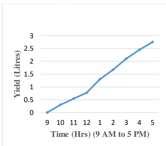
Fig. 7-Maximum yield of solar still (3 cm depth)
