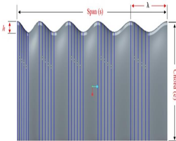
Fig: 1 (b) Tubercle wing (Top view)
