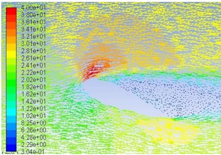
Fig: 4 (c) Velocity vector showing flow separation at AOA=20 degree for Wavy Wing Model 1 (valley) at 17.5mm from fixed end (wing root)
