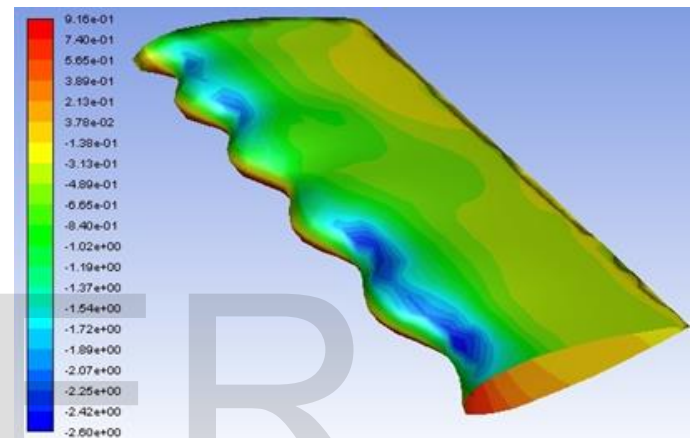
Fig: 3 Pressure distribution (static) for Re=120000 at 20 degree (c) wavy wing model 2
