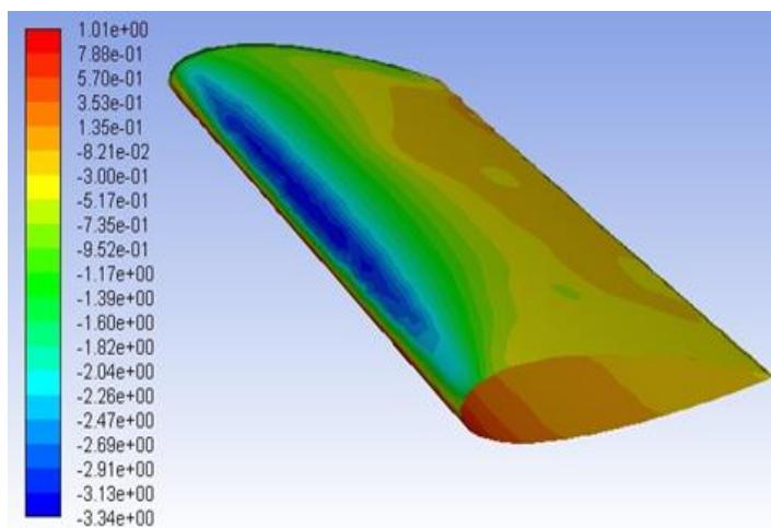
Fig:3 Pressure distribution (static) for Re=120000 at 20 degree (a) baseline model
