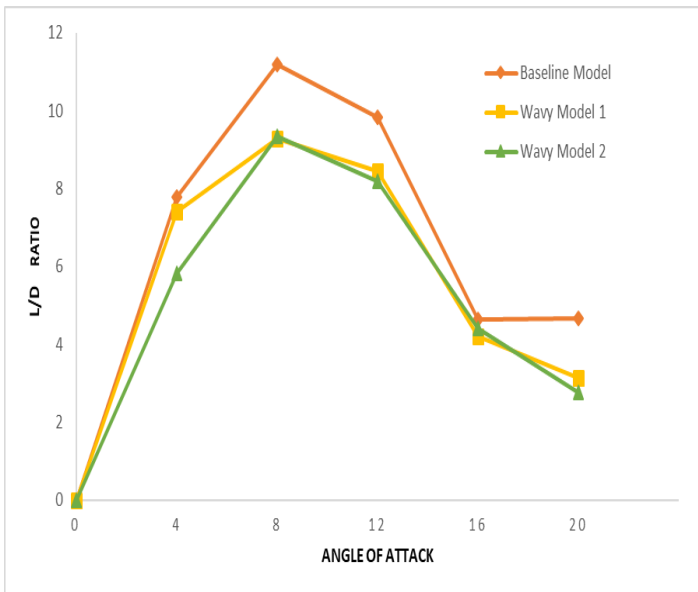
Fig: 2 L/D ratio of two tubercle wing models and baseline
