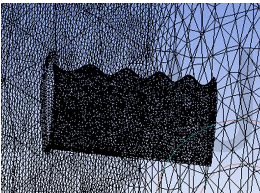
Fig: 1 (c) fluid domain meshed model
