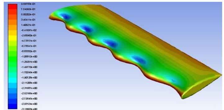
Fig: 3 Pressure distribution (static) for Re=120000 at 20 degree (b) Wavy Wing Model 1
