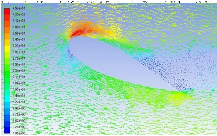
Fig: 4 (a) Velocity vector showing flow separation at AOA=20 degree for Baseline Model
