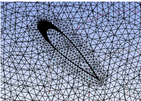
Fig:1 (d) elevation view mesh refinement in near wall region
