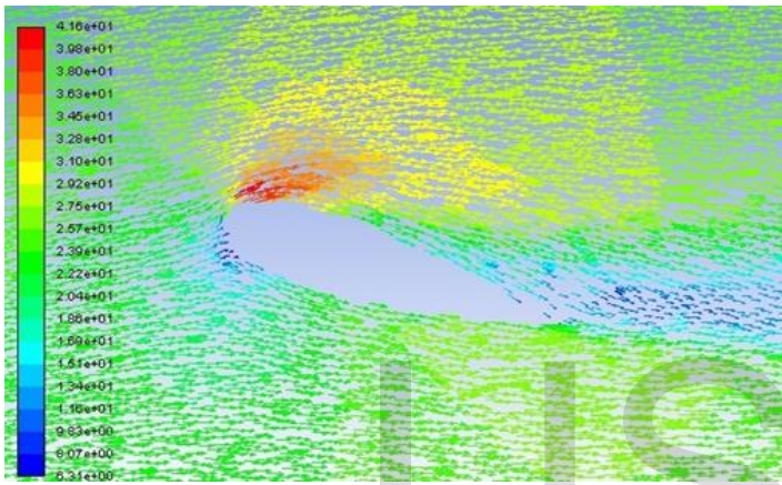
Fig: 4 (b) Velocity vector showing flow separation at AOA=20 degree for Wavy Wing Model 1 (peak) at 35mm from fixed end (wing root)
