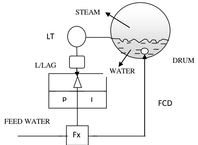
Figure-3 Single element control
