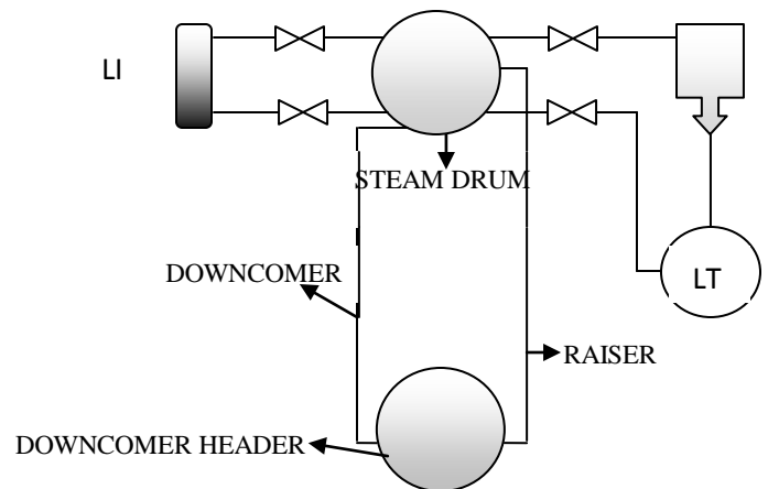
Figure-2 Boiler drum level management
