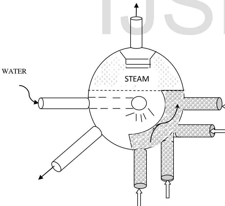
Figure-1 the water in the steam drum contains steam bubbles
