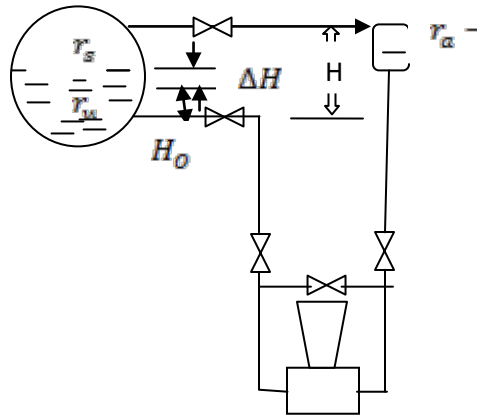
Figure-7 drum level measurement
