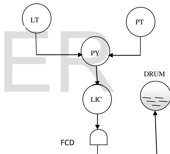
Figure-4 Single element feed water control
