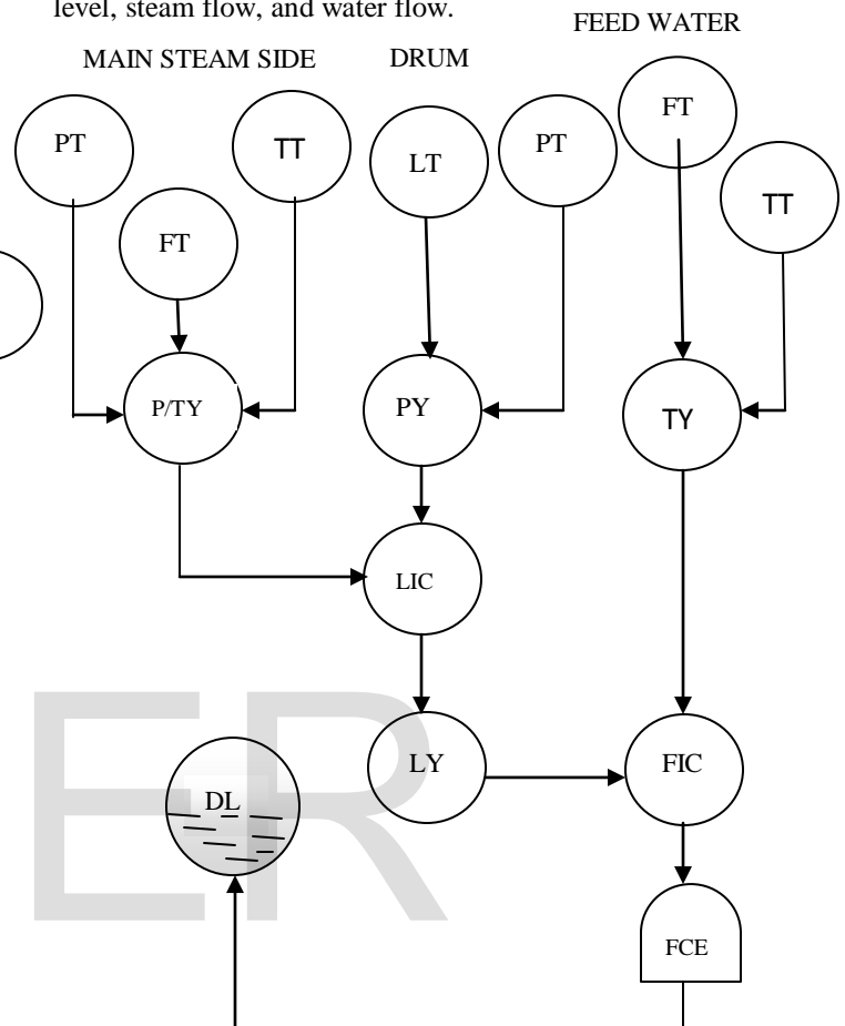
Figure-6 Three element feed water control
