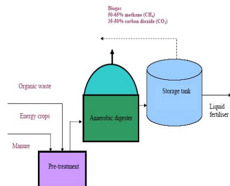
Figure 2. General schematic of an agricultural biogas plant
