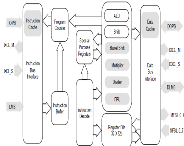
Figure 2. Proposed architecture of multiprocessor architecture.
