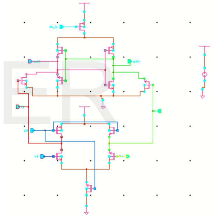
Fig2 Schematic of Double Tail Dynamic Comparator
