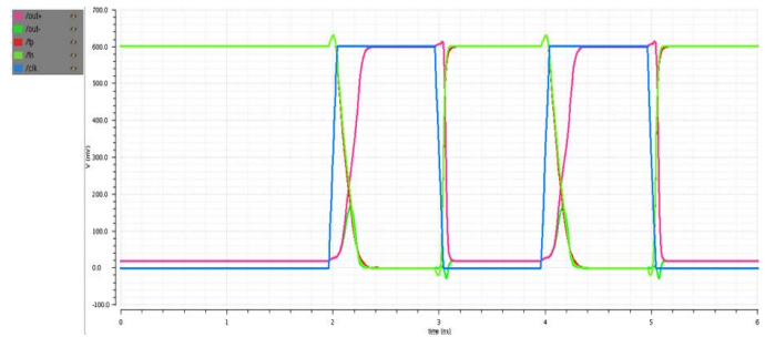
Fig5 Simulations of Double Tail Dynamic Comparator
