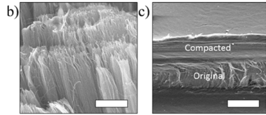
Fig 1. a) Schematic diagram of M2B (Micro-Mechanical Bending) method. b) Field Emission Scanning Electron Microscopy (FE-SEM) images of bare CNT forests view from tilted angle 30o on the side. The nanotubes are vertically aligned. Scale bar, 5 \mu\text{m} . c) FE-SEM image of CNT forest with portion being compacted. Scale bar, 15 \mu\text{m} .
