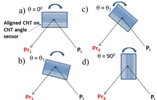
Fig. 5. Reflection of light will be measured at various angle of rotation a) 0° b) \theta_1 c) \theta_2 d) 90°. P_i = incident power of polarized light, P_{r_i} = reflected power from CNT angle sensor at \theta
