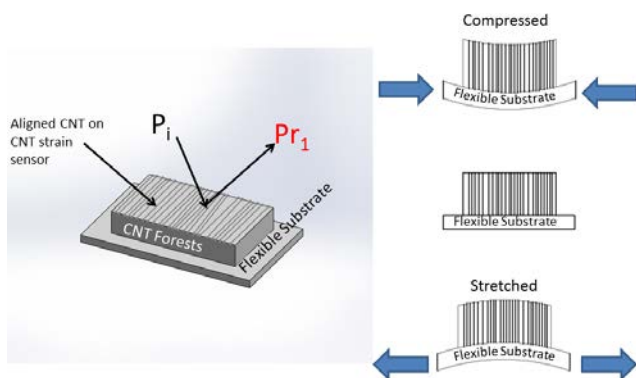
Fig. 6. Light will impinged onto the surface and reflected back (Left picture). CNT forests in compressed and expanded mode (Right image).
