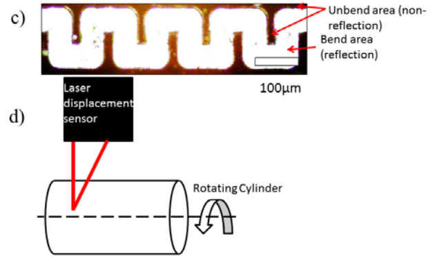
Fig. 4. (a) Conceptual diagram of the potential application of CNT forest as linear and angular encoder. As CNT forest is flexible therefore it can be used to measure both angular displacement and linear displacement if grown on a flexible substrate. b) Signal over time graph as depicted by LabView. c) Reflection from the patterned area compared to the bare CNT forest area (black area). d) Conceptual design on angular encoder.
