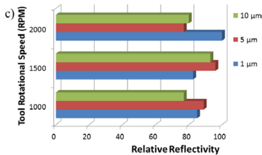
Fig 2. a) Schematic diagram of specular reflection. b) Schematic diagram of diffuse reflection. c) Graph of tool rotational speed against reflectivity.
